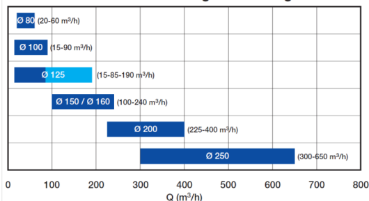
MR Modulo - Setting airflow range
